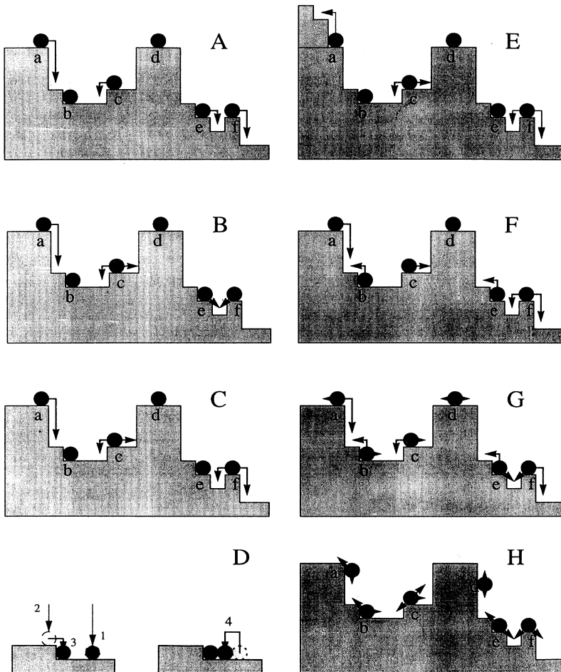
FIG. 1. Schematic configurations defining the growth rules for various models discussed in this paper in 1 + 1 dimensions. (a) Family model, (b) Wolf-Villain (WV), (c) Das Sarma-Tamborenea (DT), (d) time-dependent hopping (TDH) modification to the DT model, (e) Lai-Das Sarma (LDS), (f) larger curvature model (LC), (g) the minimal MBE model, i.e., the stochastic growth model in solid-on-solid approximation (SOS-MBE), (h) stochastic ballistic deposition model (BD). Atom a in (e), while hopping up in the modified configuration, would not move in DT, and hops down in LC.
