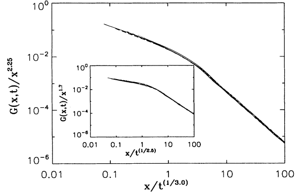
FIG. 3. Data collapse of the scaled height-height correlation function in d = 1 + 1 SOS-MBE for T = 600 K and T = 650 K (inset) with system size L = 4000 sites. Collapse is for seven times ranging from t = 32 to 2048; exponents are in Table III.
