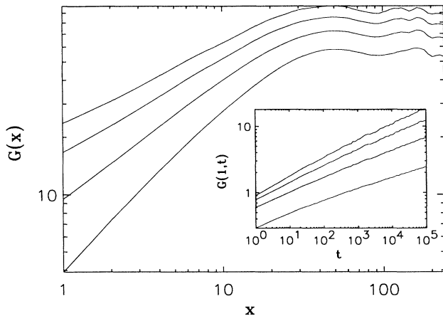
FIG. 19. Multifractal behavior of G_q(x, t) and G_q(1, t) (inset) for the TDH model with L = 500, t = 10^5 . The resulting exponents are slightly larger than in the DT model; see Table VI.
