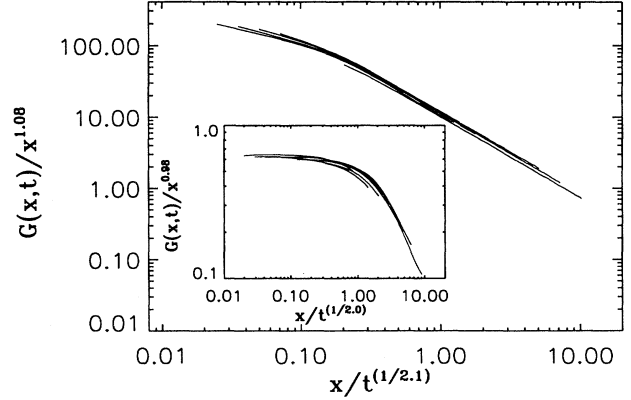
FIG. 10. Scaling collapse for the modified Family model with p = 0.05 at t = 120, 251, 524, 1096, 2290, 4786, 10\,000 for L = 200 : z = 2.1 , \alpha = 0.54 , \beta = 0.26 . Note the lack of saturation of the collapse. In the inset, the unmodified Family model is shown ( p = 1.0 ), and the scaling function quickly saturates. Same times and size used, and z = 2.0 , \alpha = 0.49 , \beta = 0.245 .
