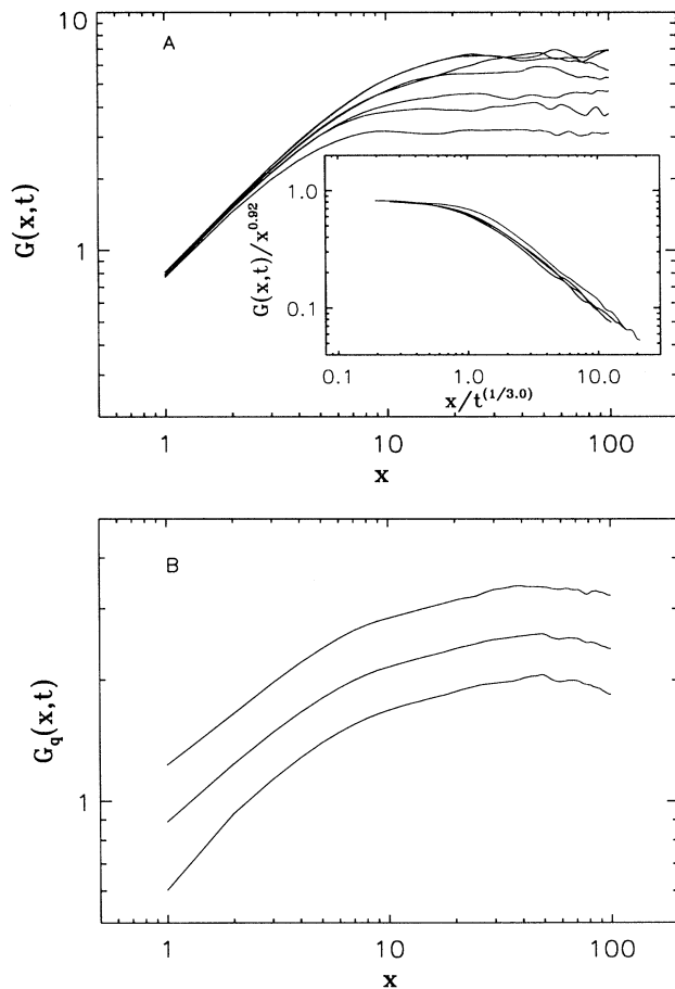
FIG. 2. (a) Correlation function G(x, t) vs x for the 3+ model in d = 3 for times t = 51, 109, 235, 505, 1084, 2324, 5000 layers (bottom to top) and L = 200 . Note the superposition of the various plots for small x . Inset: Scaling collapse G(x, t)/x^{2\alpha} vs x/t^{1/z} for t = 109, 223, 504, 1083, 5000 layers, with 2\alpha = 0.92 and z = 3.0 . (b) Plot of height-height correlation function G_q(x, t) for the 3+ model in d = 2 + 1 for different moments q = 1, 2, 4 (bottom to top). From x = 4 to 10, \alpha'_q = 0.32, 0.31, 0.31 for q = 1, 2, 4 , respectively. L = 200, t = 5000 layers.
