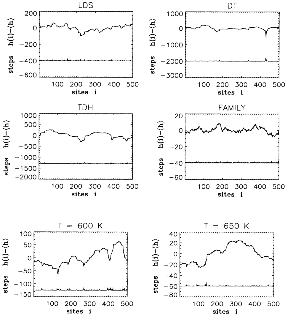
FIG. 9. Morphologies of several dynamical models for L = 500 : LDS model for t = 1 \times 10^5 layers; DT model for t = 1 \times 10^6 layers; TDH model after t = 1 \times 10^6 ; Family model at t = 1 \times 10^6 . The lower plot in each figure shows a trace of the step height at each site. Note the very different vertical scale in the various cases as dictated by the widely changing scaling exponents. We also show saturated ( t = 131072 layers) SOS-MBE morphologies for T = 600 and 650 K in 1+1 dimensions for L = 500 . We include the step-height distributions for comparison of the intermittent properties of the two classes of models.
