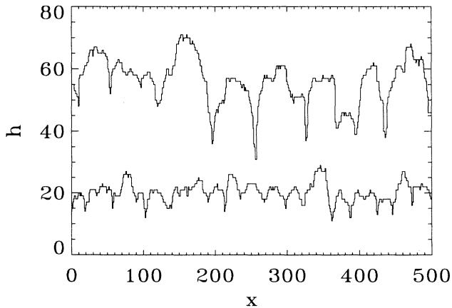
FIG. 12. Morphology of the SOS-MBE surface at t = 100, 4000 monolayers at T = 600 K, L = 4000 .
