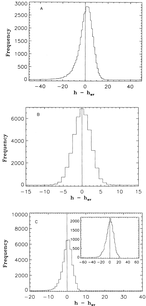
FIG. 14. Height distribution functions around the mean for L = 200 in the (a) DT, (b) 3+, and (c) d = 2 + 1, T = 600 K SOS-MBE models [the inset of (c) gives d = 1 + 1, L = 1000, T = 600 K results]. Only the normally scaling 3+ model has a symmetric distribution function, while a tail for large, negative height fluctuations exists in all other cases.
