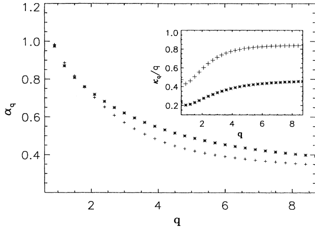
FIG. 16. Expanded q dependence of the exponents \alpha'_q and \kappa(q)/q (inset) for the LDS (*) and DT (+) models. Notice the close correspondence of \alpha'_q for the two models while the plateaus of \kappa(q)/q differ by about 0.5, expected by comparison with continuum equations.
