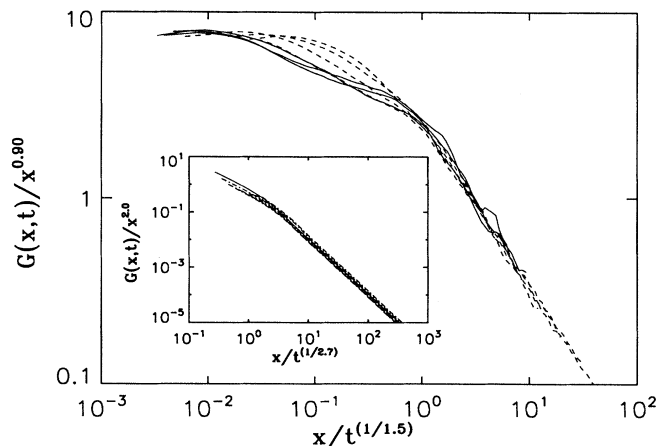
FIG. 6. Data collapse of the late time behavior of the correlation function in the BD model at T = 600 K with L = 4000 , for six times ranging from t = 128 to 4096 : 2\alpha = 0.90, z = 1.5 . The inset shows data from the same simulation, at seven times from t = 0.5 to 64 , but now 2\alpha = 2.0 and z = 2.7 , consistent with the idea of a SOS transient in the BD model.
