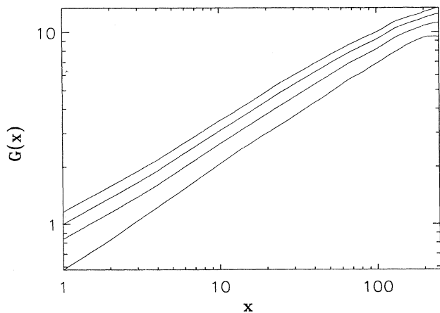
FIG. 17. Correlation function G_q(x, t = 1 \times 10^6) vs x for the Family model with L = 500 . The near constancy of the slopes for q = 1, 2, 3, 4 (from bottom to top) indicates the presence of self-affine scaling, for \alpha'_1 = 0.53 \pm 0.02 , very close to \alpha'_4 = 0.48 \pm 0.02 .
