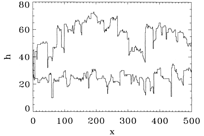
FIG. 13. Morphology of the BD surface at t = 100, 4000 monolayers at T = 600 K, L = 4000 .
