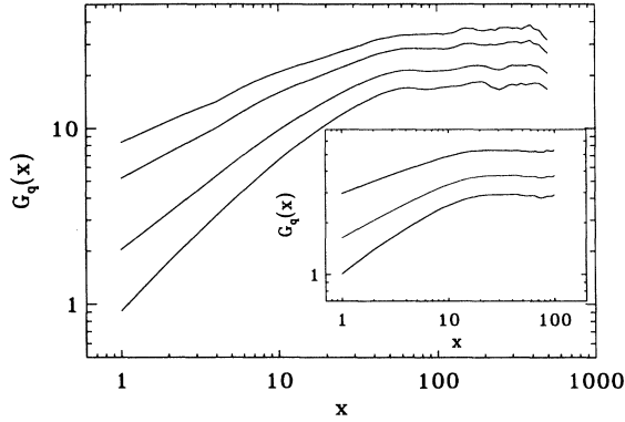
FIG. 11. Multi-affine behavior of the correlation function G_q(x,t) for the SOS-MBE models in 1+1 dimensions, T = 600 K, L = 1000 after 8192 layers grown. The moments q = 1, 2, 4, 6 are displayed (from bottom). Inset: 2+1 dimensions, T = 600 K, L = 500 after 1000 layers grown. The moments q = 1, 2, 4 are shown from bottom to top. The variation in initial slope here indicates multi-affinity.
