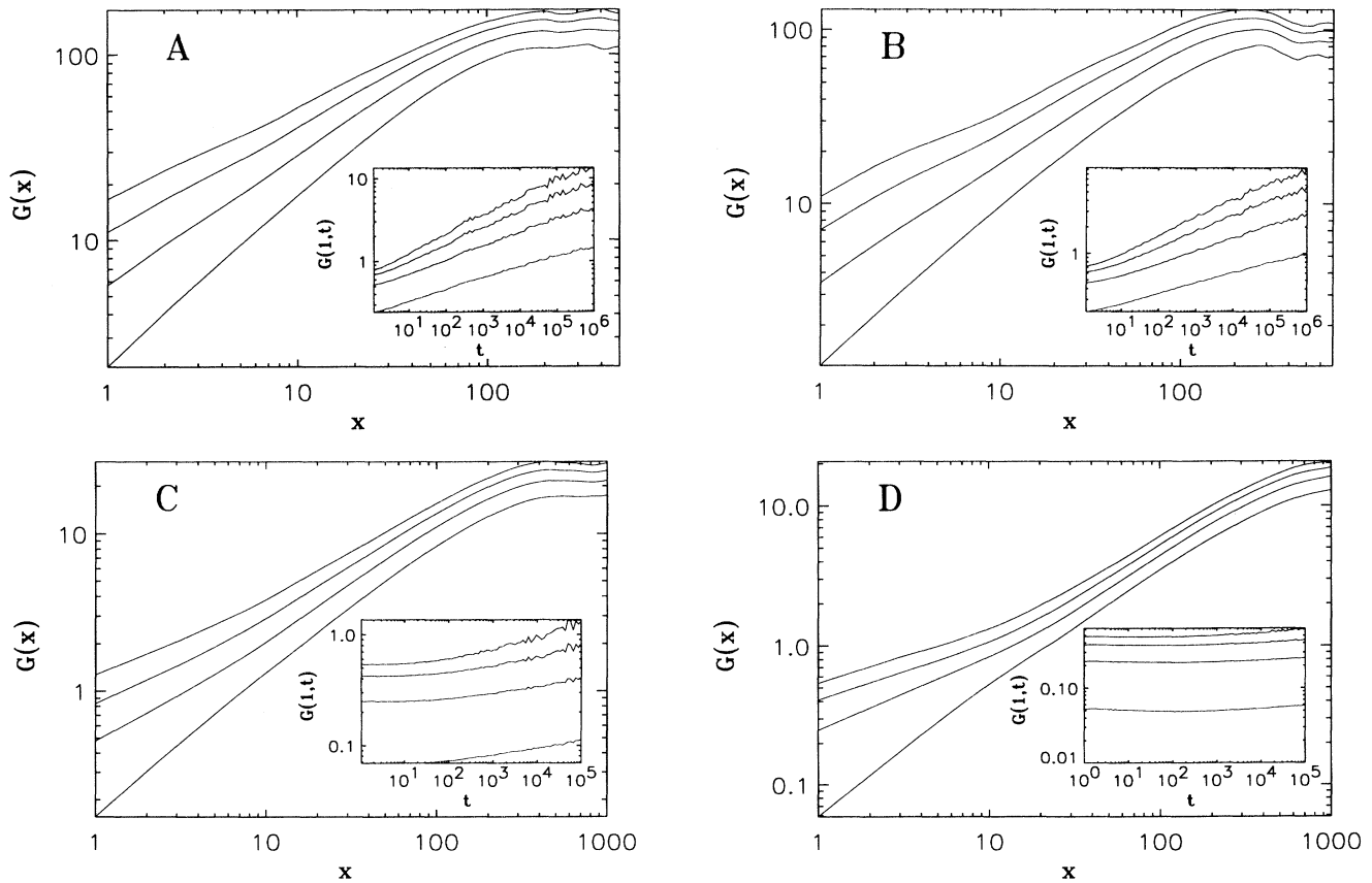
FIG. 18. Multifractional behavior of G_q(x, t) and G_q(1, t) (inset) for the DT model with variable diffusion length. (a) D = 2 , L = 1000 , t_{\max} = 1 \times 10^6 , (b) D = 3 , L = 1500 , t_{\max} = 1 \times 10^6 , (c) D = 10 , L = 5000 , t_{\max} = 1 \times 10^5 , (d) D = 20 , L = 10000 , t_{\max} = 1 \times 10^5 . To measure \alpha'_q , we extract the slope from the x > D region to avoid the finite size effects seen for small x at large D . \kappa(q)/q is measured in the range 10^4 – t_{\max} . The exponents found are tabulated in Table VI. Note that D/L is kept constant.
