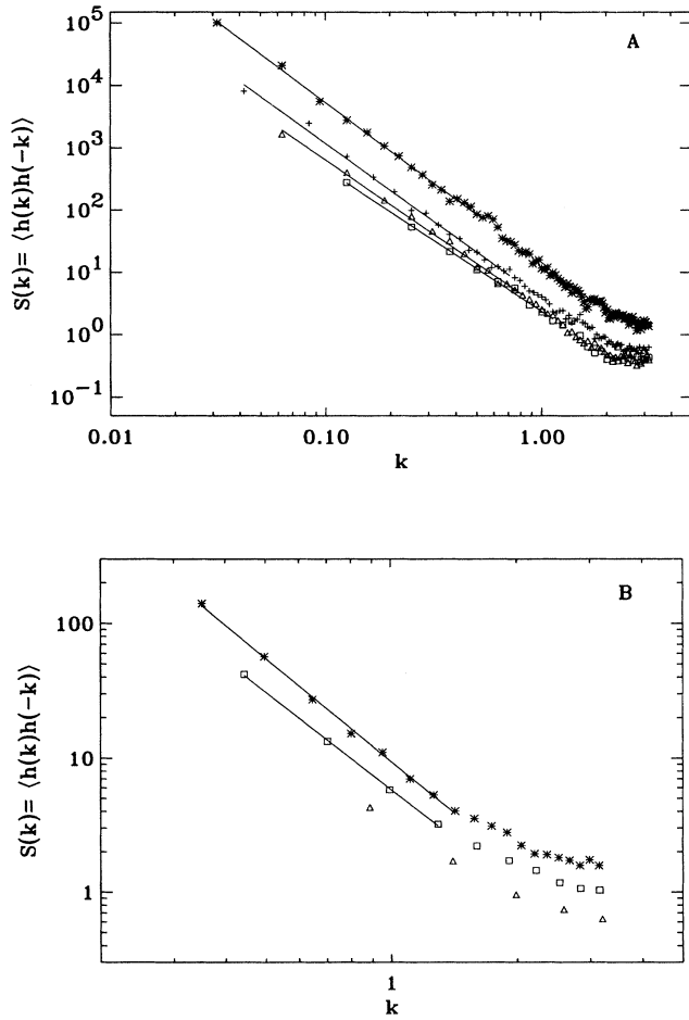
FIG. 7. Plot of the structure factor S(k) at T = 600 K for various system sizes for SOS-MBE in (A) 1 + 1 and (B) 2 + 1 . The system sizes in d = 1 + 1 are L = 50 ( \square ), 100 ( \triangle ), 150 ( + ), 200 ( * ), and for d = 2 + 1 , L = 10 ( \triangle ), 20 ( \square ), 40 ( * ). Slopes for the largest systems are 2.6 \pm 0.05 and 2.55 \pm 0.10 in d = 1 + 1, 2 + 1 , respectively.
