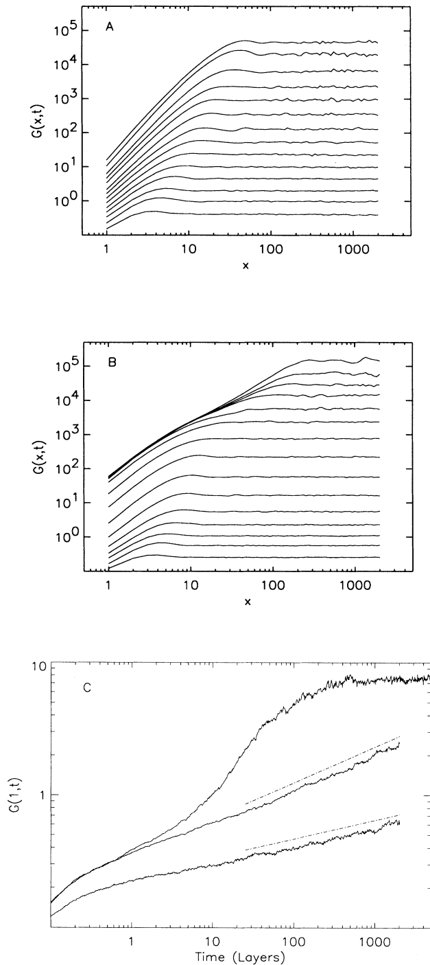
FIG. 5. Raw correlation function vs distance x for times t = 2^j, j = -2, -1, \dots, 11, 12 in the SOS-MBE model (a) and BD model (b) at T = 600 K in d = 1 + 1 ( L = 4000 ). Note the different behavior for small x as a function of time; compare these as well with Fig. 2(a) for the 3+ model. (c) G(1,t) , or equivalently, the mean square slope of the interface, versus time for BD (top) and SOS at T = 600 K (middle), and SOS at T = 650 K (bottom). The slopes equal to \kappa/z of the dashed lines are 0.27 \pm 0.02 and 0.14 \pm 0.02 for the T = 600 and 650 K SOS cases, respectively. (Compare with \kappa/z_{600} = 0.32 and \kappa/z_{650} = 0.19 from Table IV.)
