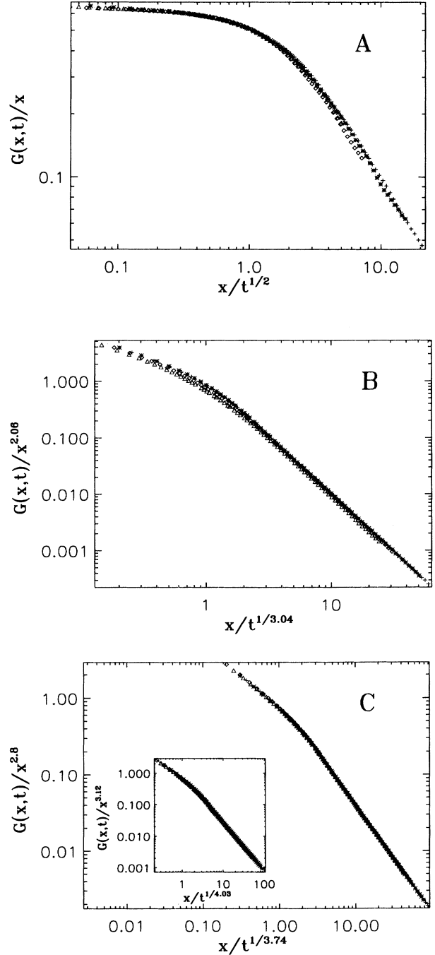
FIG. 8. Scaling collapses displaying G(x,t)/x^{2\alpha} vs y = x/t^{1/z} for various dynamical models for t = 524, 1060, 2100, 4900, 10000 for a system size of L = 10^4 : (a) Family, (b) LDS, and (c) DT (TDH in inset). Notice how only the Family model saturates at small y , all other models are increasing for decreasing y .
