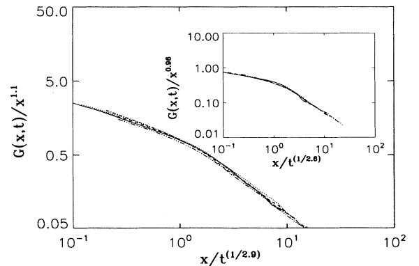
FIG. 4. Data collapse of the scaled height-height correlation function in d = 2 + 1 SOS-MBE for T = 600 K and T = 640 K (inset) with a system of L = 500 \times 500 sites. Collapse is for five times ranging from t = 45 to 1000; exponents are in Table III.
