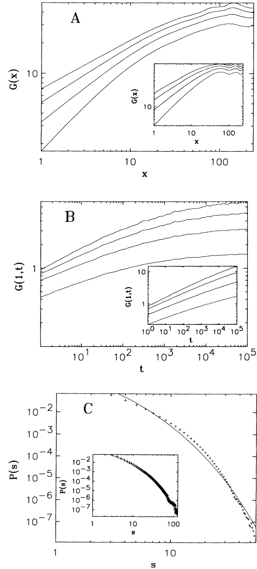
FIG. 15. Comparison of multifractal scaling properties in the LDS and DT (inset) models. (A) Correlation functions G_q(x, t = 1 \times 10^5) vs x for q = 1, 2, 3, 4 from bottom to top, where the slope for x = 1 - 10 gives \alpha'_q ( L = 500 ). (B) The average step height G_q(1, t) vs t , where the slope for 1 \ll t^{1/z} \ll L is \kappa(q)/qz . These results are ten-run averages, and the q dependence of the exponents extracted appears in Table V. (C) P(s) vs the step size s for L = 25 , sampling the saturation regime 10^5 times to acquire sufficient statistics. The solid line is a fit to a stretched exponential C \exp^{-as^\delta} , where \delta = 0.47 (0.42) for LDS (DT).
